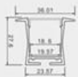
Model: ZJD-LS2428B Size:Lx36.01x27.6mm PCB:19.57mm
