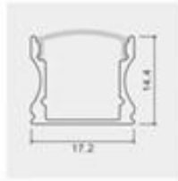
Model: ZJD-LS1714 Size: Lx17.2x14.4mm PCB: 12mm
