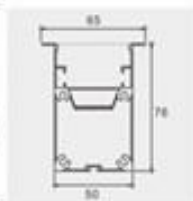
Model: ZJD-LS5076B Size:Lx65x76mm PCB:29mm
