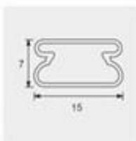
Model: ZJD-LS1507 Size: Lx15x7mm PCB: 12mm
