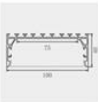
Model: ZJD-LS10040 Size: Lx100x40mm PCB: 75mm
