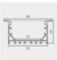
Model: ZJD-LS7040B Size:Lx86x40mm PCB:45mm
