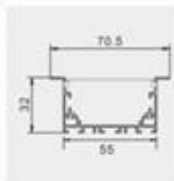
Model: ZJD-LS5532B Size:Lx70x32mm PCB:36mm
