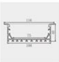
Model: ZJD-LS10040B Size:Lx116x40mm PCB:75mm
