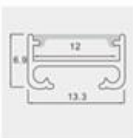
Model: ZJD-LS1307B Size: Lx13.3x6.9mm PCB: 12mm
