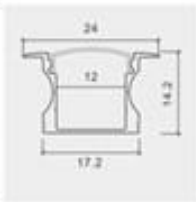
Model: ZJD-LS1714B Size:Lx24x14.2mm PCB:12mm
