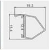
Model: ZJD-LS1915 Size: Lx19.3x15.4mm PCB: 12mm
