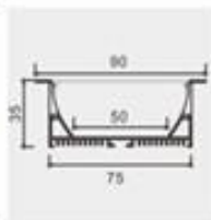
Model: ZJD-LS7535B Size:Lx90x35mm PCB:50mm
