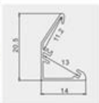
Model: ZJD-LS2114 Size:Lx20.5x14mm PCB:12mm
