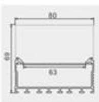
Model: ZJD-LS8069 Size: L80x69mm PCB: 63mm
