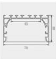
Model: ZJD-LS7040 Size: Lx70x40mm PCB: 45mm
