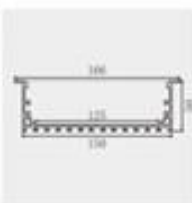
Model: ZJD-LS15050B Size:Lx166x50mm PCB:125mm
