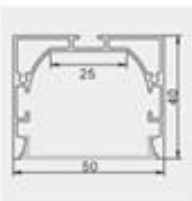
Model: ZJD-LS5040 Size: Lx50x40mm PCB: 25mm
