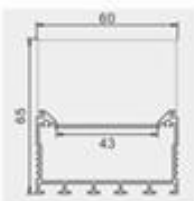
Model: ZJD-LS6065 Size: Lx60x65mm PCB: 43mm
