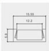
Model: ZJD-LS1606 Size: Lx15.55x5.9mm PCB: 12mm
