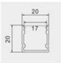
Model: ZJD-LS2020 Size:Lx20x20mm PCB:17mm
