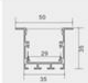
Model: ZJD-LS3535B3 Size:Lx50x35mm PCB:26mm
