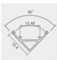
Model: ZJD-LS1616 Size: Lx15.8x15.8mm PCB: 12.4mm
