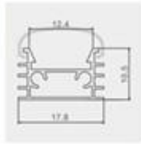
Model: ZJD-LS1811 Size: Lx17.8x10.5mm PCB: 12mm
