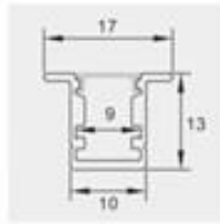
Model: ZJD-LS1013B Size: Lx17x13mm PCB: 8mm
