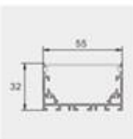
Model: ZJD-LS5532 Size:Lx55x32mm PCB:36mm
