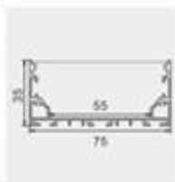
Model: ZJD-LS7535C Size:Lx75x35mm PCB:54mm
