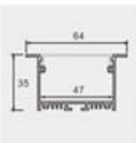
Model: ZJD-LS5035B Size:Lx64.2x35mm PCB:46.5mm
