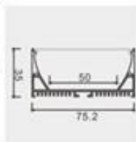
Model: ZJD-LS7535 Size:Lx75.2*35mm PCB:50mm
