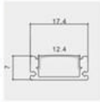
Model: ZJD-LS1707 Size: Lx17.4x7mm PCB: 12mm
