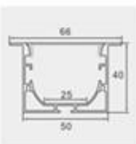
Model: ZJD-LS5040B Size:Lx66x40mm PCB:25mm
