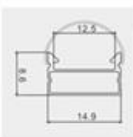
Model: ZJD-LS1509 Size: Lx14.9x8.6mm PCB: 12mm
