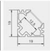
Model: ZJD-LS1919 Size: Lx19x19mm PCB: 12mm
