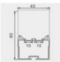
Model: ZJD-LS4060 Size: Lx40x60mm PCB: 10mm
