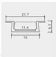
Model: ZJD-LS1606B Size:Lx21.7x5.7mm PCB:11mm
