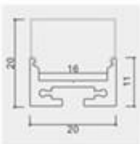
Model: ZJD-LS2020C Size:Lx20x20mm PCB:16mm
